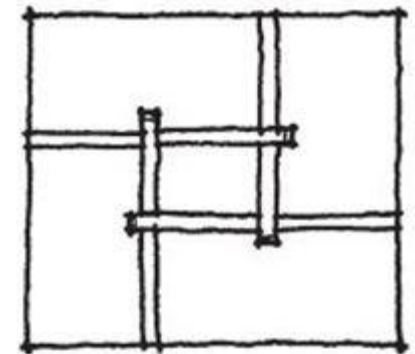
Reciprocal frame
