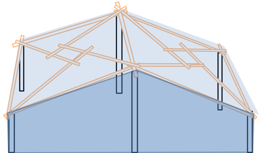
SIX POSTS FOR THE DOUBLE ELEVATED RSK
